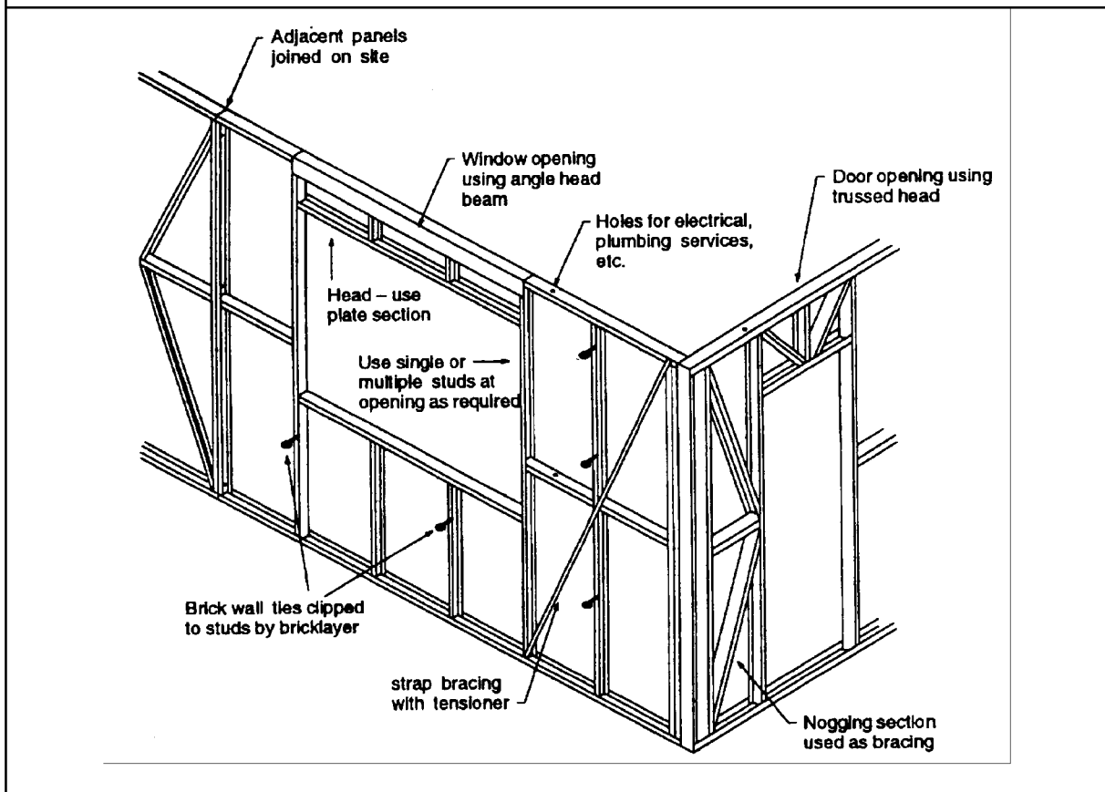
Figure 3.4.2.3 TYPICAL BRACING SYSTEM DETAILS
