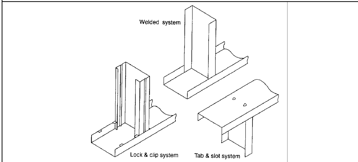
Figure 3.4.2.2 TYPICAL WALL FRAMING AND SECTION MEMBERS
