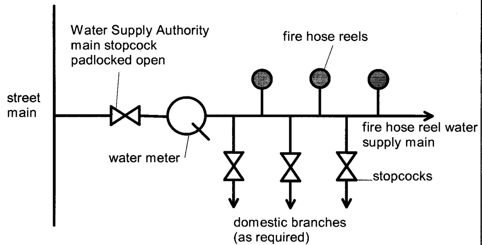
Figure E1.4 WATER SUPPLY RETICULATION: COMBINED SERVICES
