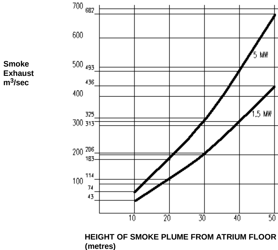
Figure 3.4 SMOKE EXHAUST RATE
